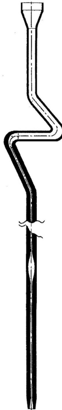
FIG. 1 Houillon Tube Schematic Diagram
